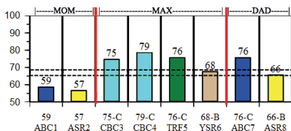
Attention Problems
